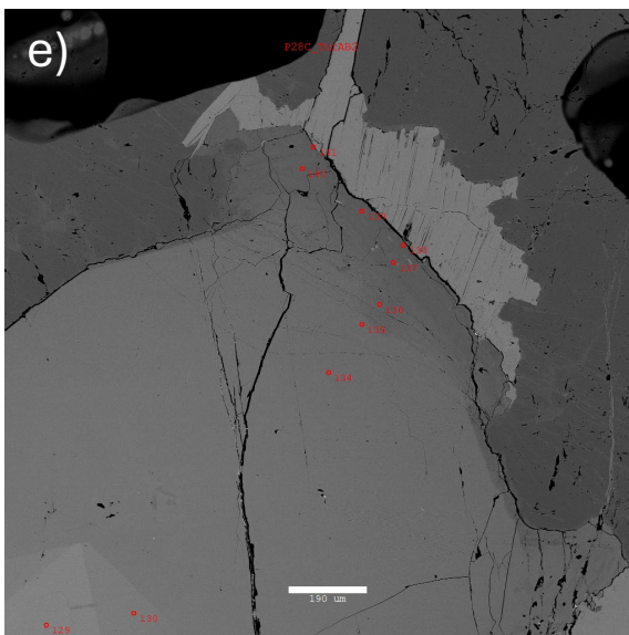
Appendix B.4 Backscatter electron (BSE) images of tourmalines from central zone, distal tourmaline subzone
