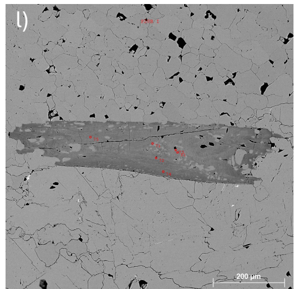
Appendix B.4 cont. Backscatter electron (BSE) images of tourmalines from central zone, distal tourmaline subzone
