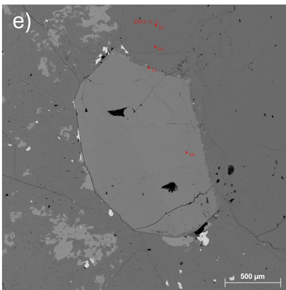
Appendix B.2 Backscatter electron (BSE) images of tourmalines from intermediate zone, graphic subzone
