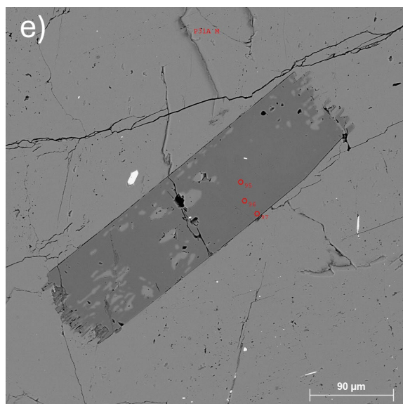
Appendix B.5 Backscatter electron (BSE) images of tourmalines from central zone, core subzone
