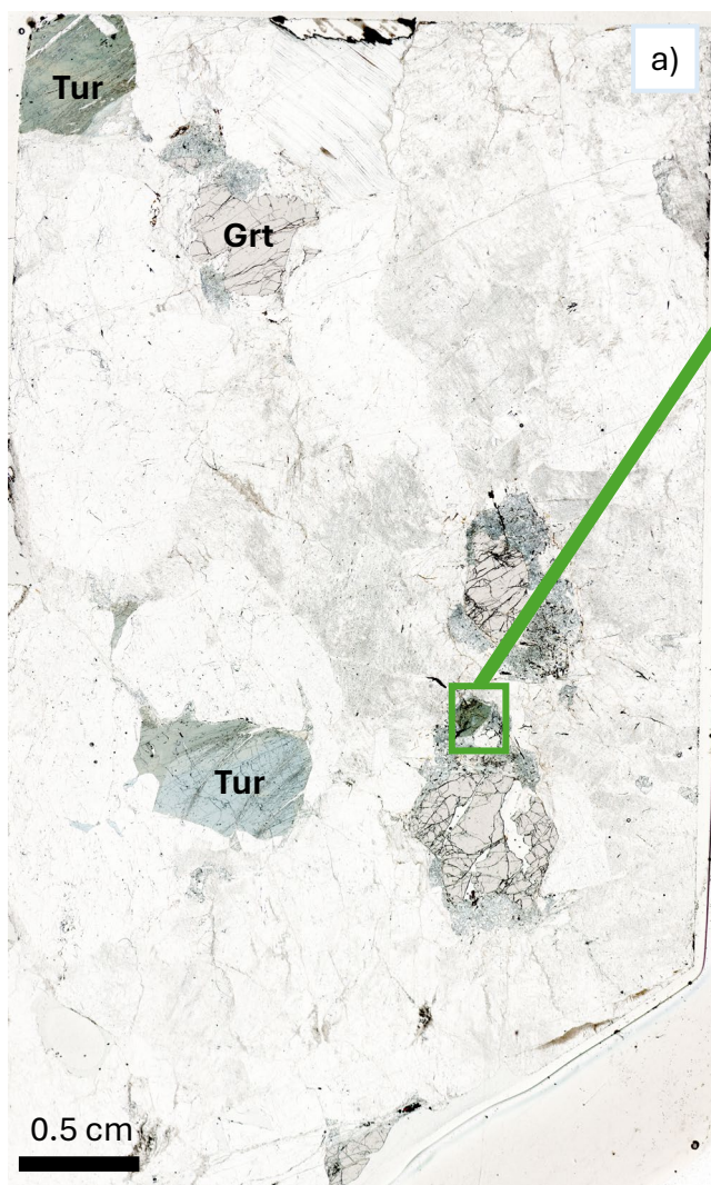
Appendix A.3 Thin section images of intermediate zone, overgrowth subzone tourmalines a) Thin section PFG2A in PPL, Tur = tourmaline, Grt = garnet, Qz = quartz, b) Zoomed in PPL image of tourmaline from PFG2A showing magmatic green core and colourless metasomatic Tur + Qz intergrowth rim, c) XPL image of same tourmaline, d) XPL image of Grt surrounded by metasomatic mica and Tur + Qz .
