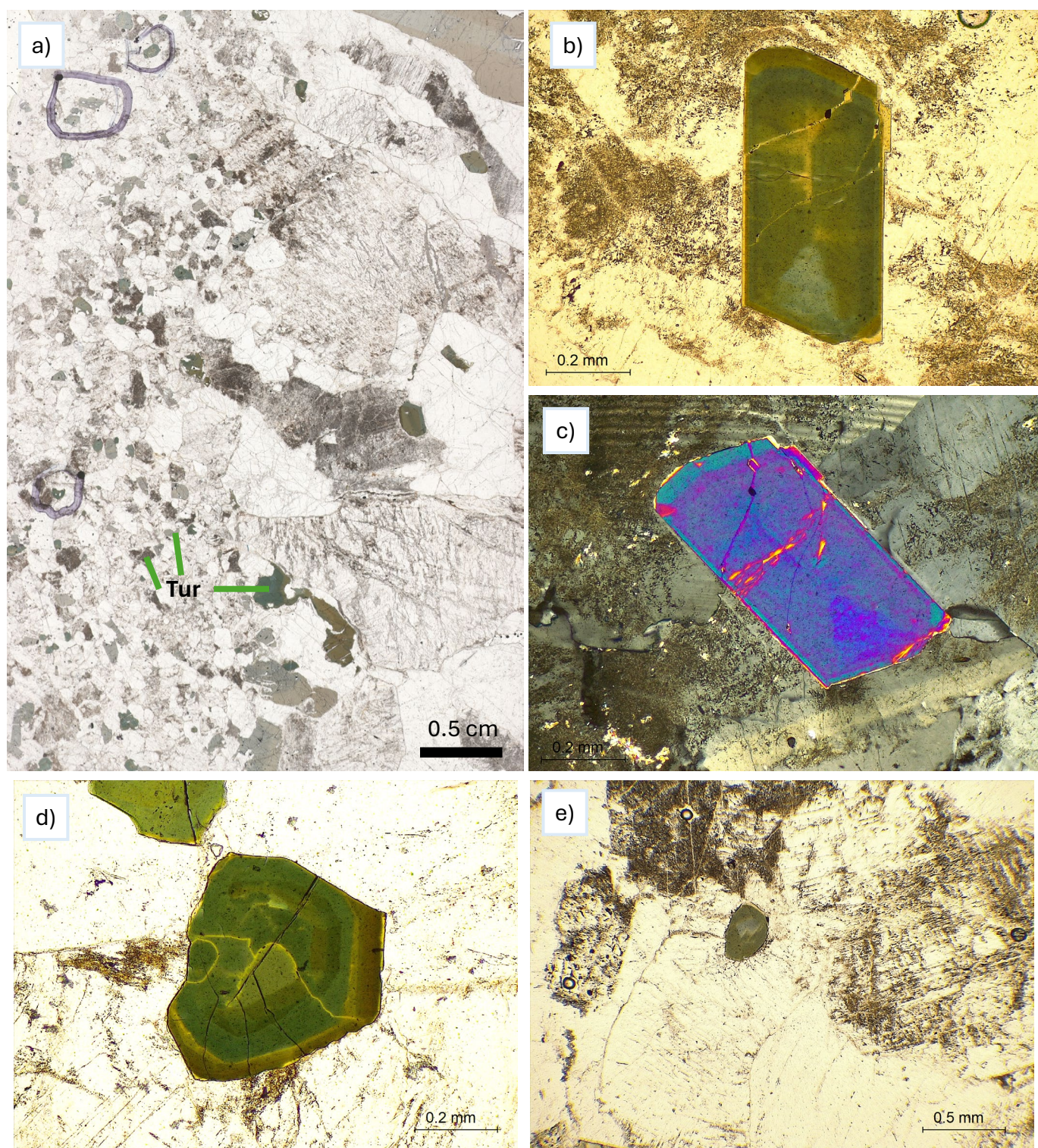
Appendix A.2 Thin section images of intermediate zone, graphic subzone tourmalines a) Thin section PFS1C in PPL, b) Tourmaline in PPL, thin section PFS1A, c) Tourmaline in XPL, thin section PFS1A, d) zoned tourmaline with clear elbaite rim, thin section PFS1A in PPL, e) tourmaline in PPL from thin section PFS1A.
