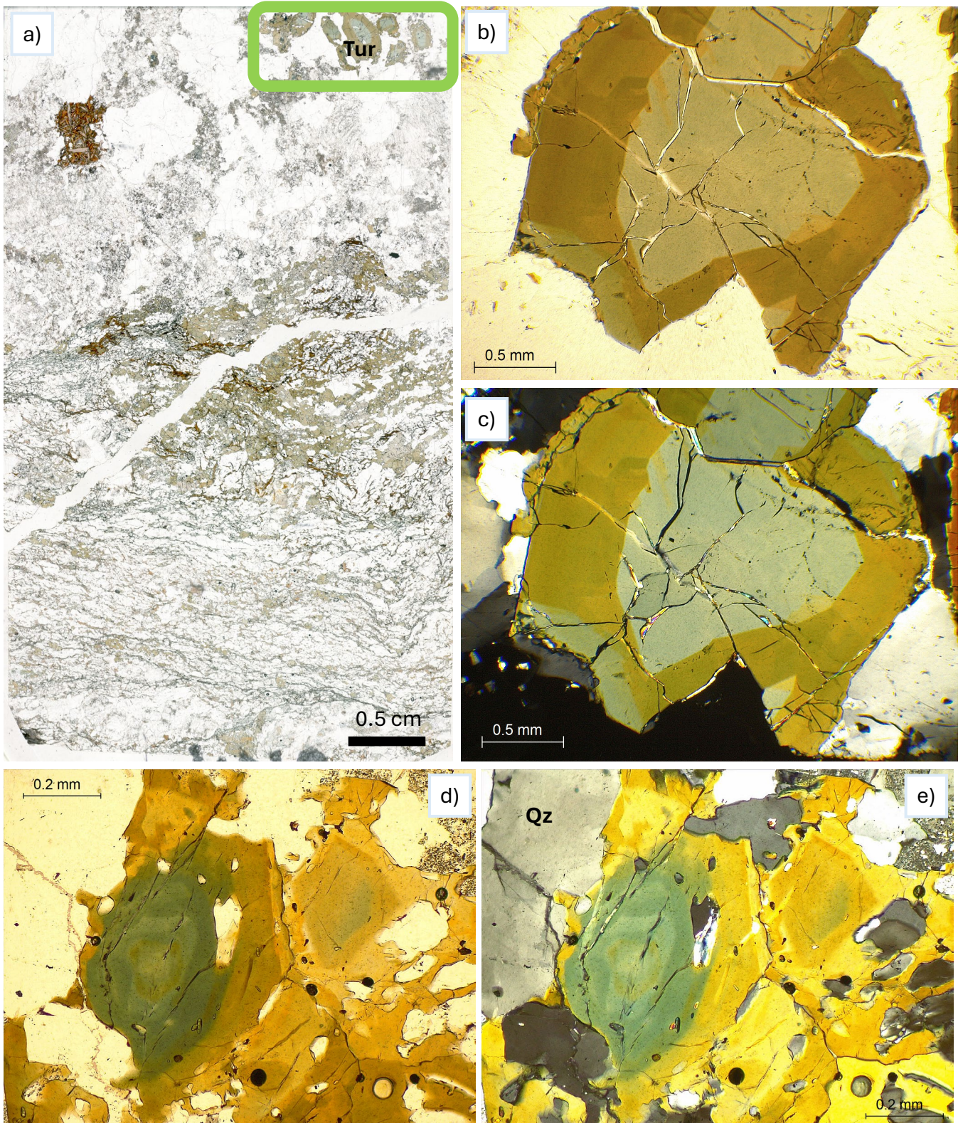
Appendix A.1 Thin section images of border zone tourmalines a) Thin section PFL7B plane-polarized light (PPL) scan, tourmalines circled in green. b) Zoomed in PPL image of tourmaline in PFL7B, c) Cross polarized light (XPL) image of tourmaline in PFL7B, d) Thin section P24B PPL tourmaline, e) XPL image of tourmaline in P24B. Tur = tourmaline, Qz = quartz.
