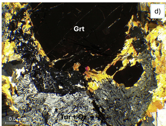
Appendix A.3 Thin section images of intermediate zone, overgrowth subzone tourmalines a) Thin section PFG2A in PPL, Tur = tourmaline, Grt = garnet, Qz = quartz, b) Zoomed in PPL image of tourmaline from PFG2A showing magmatic green core and colourless metasomatic Tur + Qz intergrowth rim, c) XPL image of same tourmaline, d) XPL image of Grt surrounded by metasomatic mica and Tur + Qz .
