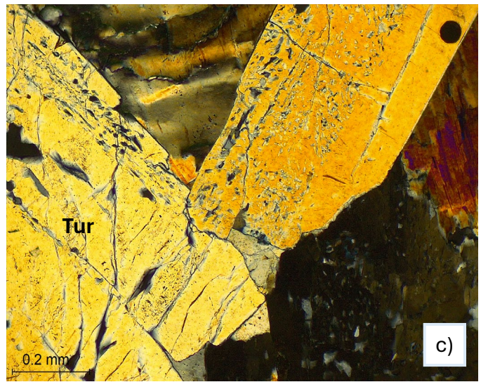
Appendix A.4 Thin section images of central zone, distal tourmaline subzone tourmalines a) Thin section PFL12A in PPL, b) Zoomed in PPL image of tourmaline from thin section PFL12A, c) XPL image of same tourmaline, d) PPL image of magmatic fluor-elbaite from distal tourmaline subzone from thin section P28C.
