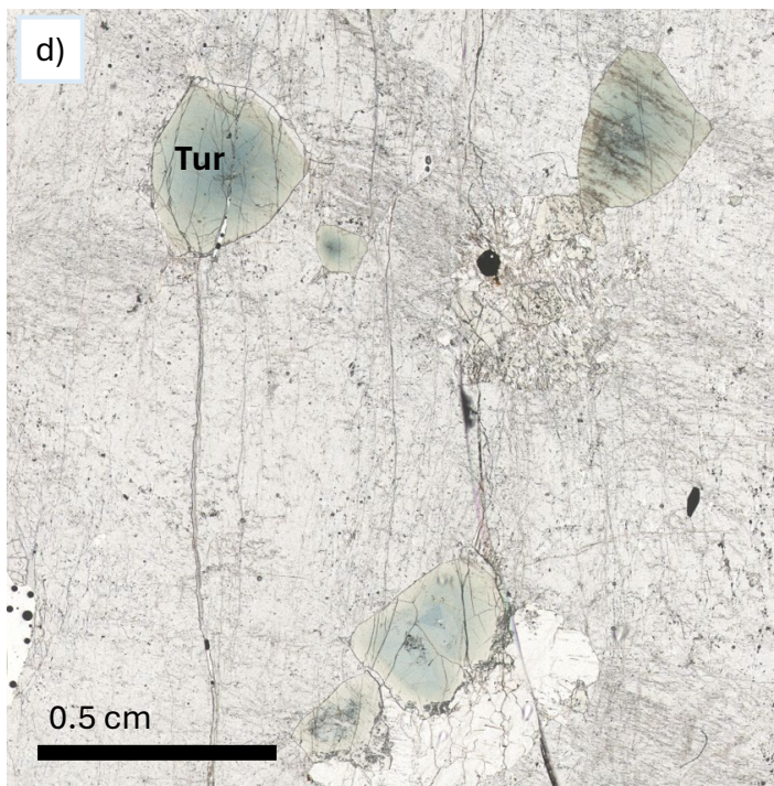
Appendix A.4 Thin section images of central zone, distal tourmaline subzone tourmalines a) Thin section PFL12A in PPL, b) Zoomed in PPL image of tourmaline from thin section PFL12A, c) XPL image of same tourmaline, d) PPL image of magmatic fluor-elbaite from distal tourmaline subzone from thin section P28C.
